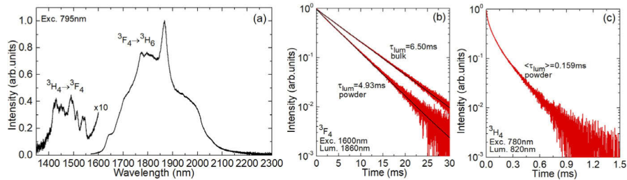
Fig. 7. Near-infrared emission properties of the Tm:CLTGG crystal: (a) luminescence spectrum, \lambda_{exc} = 795 \text{ nm} ; (b,c) luminescence decay curves from the (b) ^3F_4 and (c) ^3H_4 Tm 3+ states.
