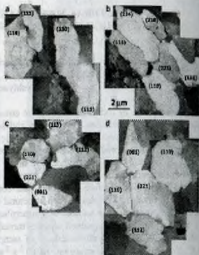
Figure 2. Dark field TEM image of grain structure in Al-Sc-Li-Zr alloy. Tension at 370°C. Strain - 110% (a), 300% (b), 900% (c), 1200% (d). Indexes of zone axes for some grains are indicated.
