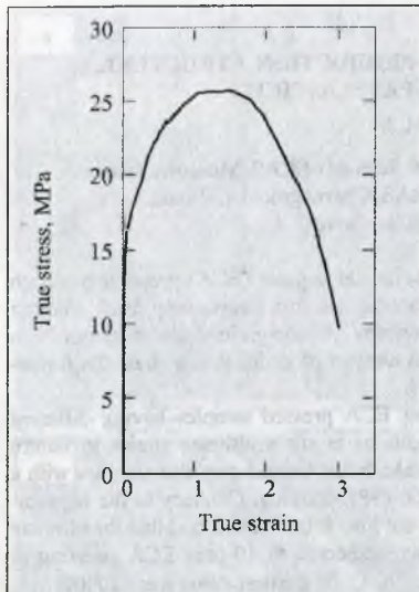
Figure 1. True stress vs true strain. Al-Sc-Li-Zr alloy.
